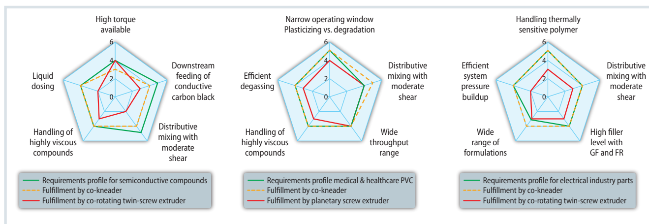
Fig. 6. Technology comparison: degree of fulfillment of requirements for manufacturing a) semiconductive compounds for high-voltage cables, b) PVC compounds for medical technology, and c) parts for the electrical industry, each in comparison with a competing compounding technology; GF = glass fibers, FR = flame retardants [5] Source: Buss; graphic: © Hanser
